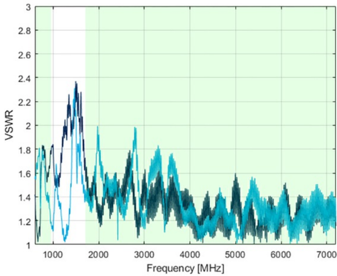
TYPICAL VSWR CURVE 4G/5G/WIFI PORT 1 & 2
