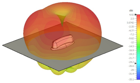
800 MHz, side view
