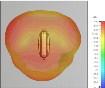
1800 MHz, top view
