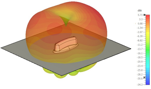
900 MHz, side view
