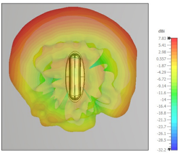
3600 MHz, top view
