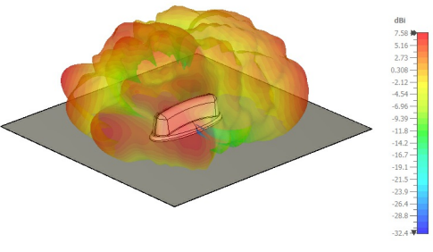
6000 MHz, side view
