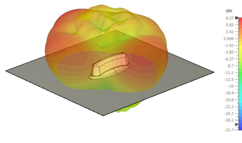
2100 MHz, side view
