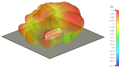
5000 MHz, side view
