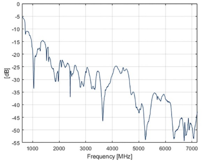
TYPICAL ISOLATION CURVE 4G/5G/WIFI BETWEEN PORT 1 & 2
