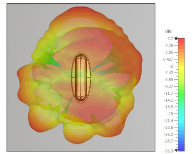
5000 MHz, top view
