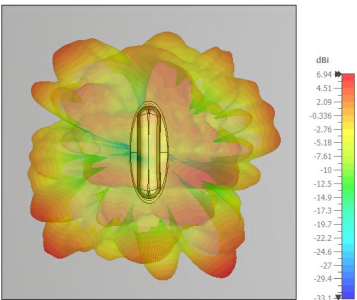
7000 MHz, top view
