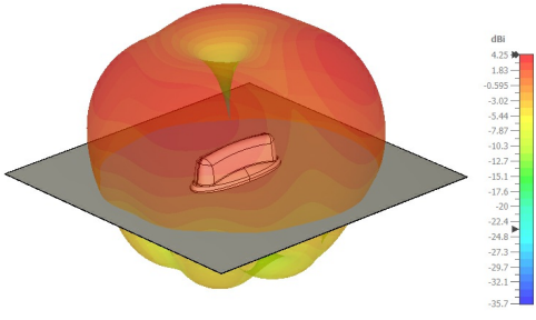
650 MHz, side view
