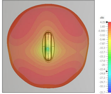
650 MHz, top view
