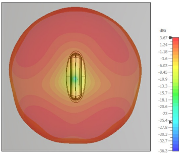
700 MHz, top view
