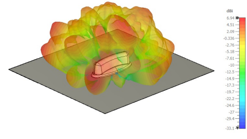
7000 MHz, side view
