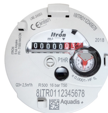
Aquadis+ Register available in plastic and mineral glass versions
